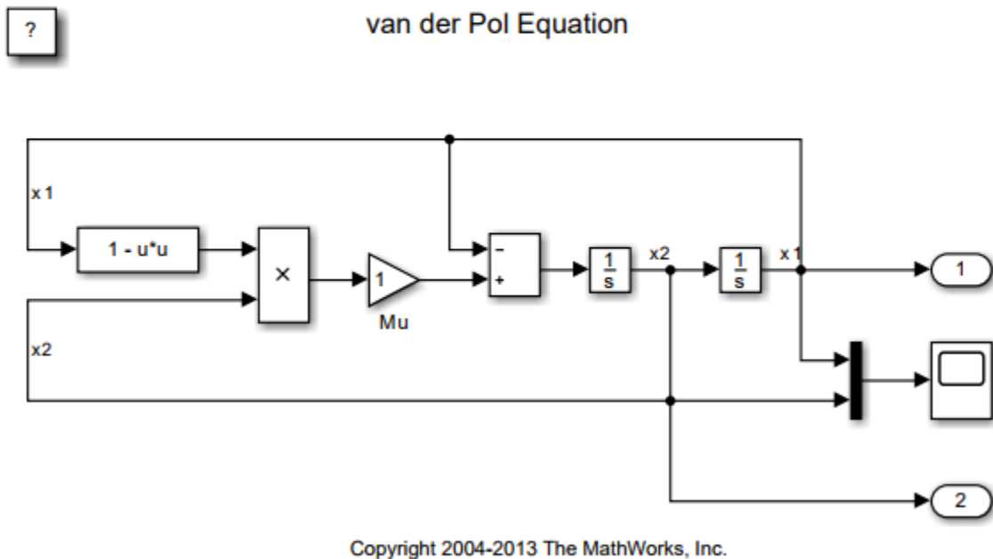
Figure 1.1. The van der Pol Equation
